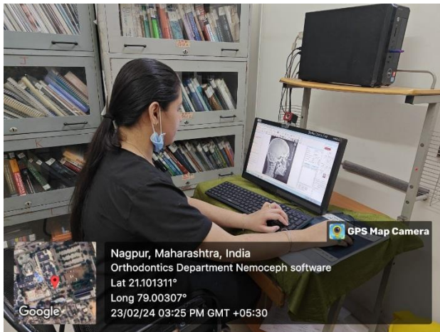
Nemoceph software.
